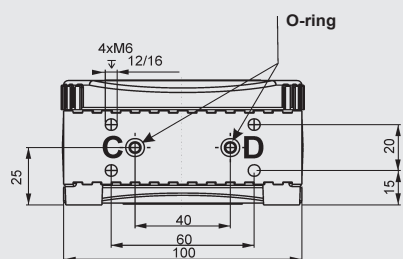
Flange connection
